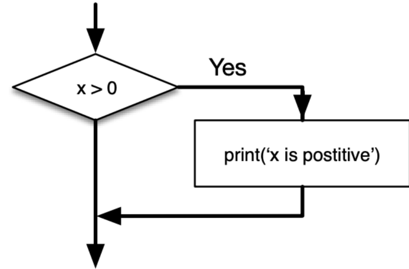
Figure 3.1: If Logic
