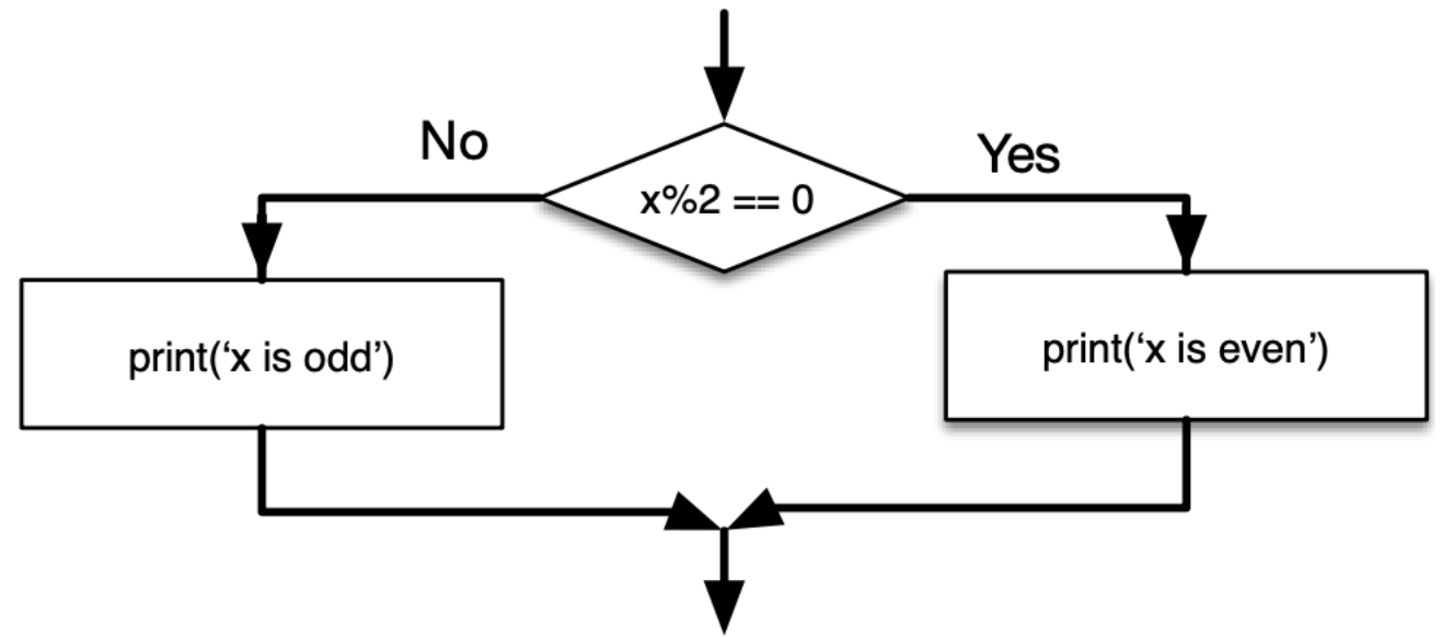
Figure 3.2: If-Then-Else Logic
