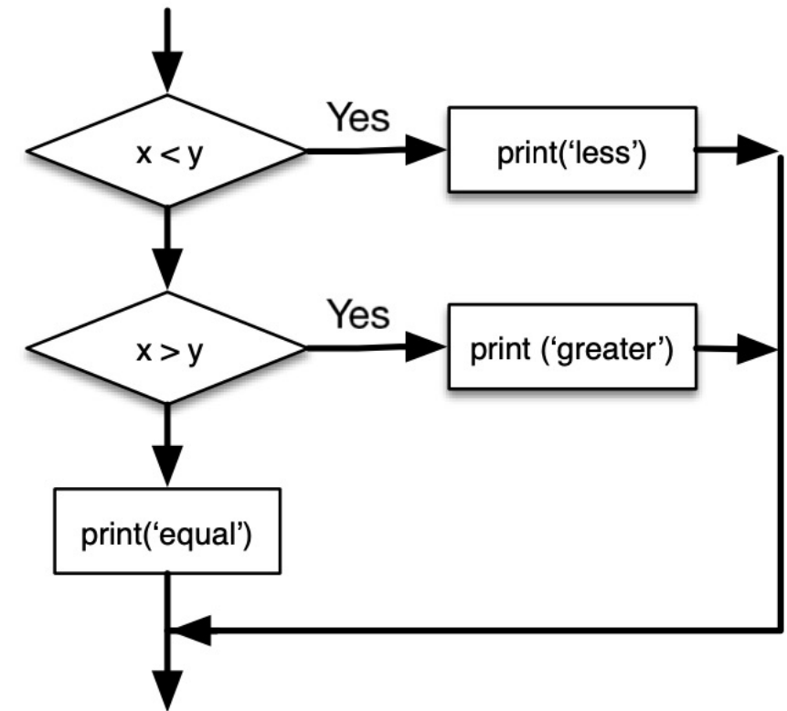
Figure 3.3: If-Then-ElseIf Logic
